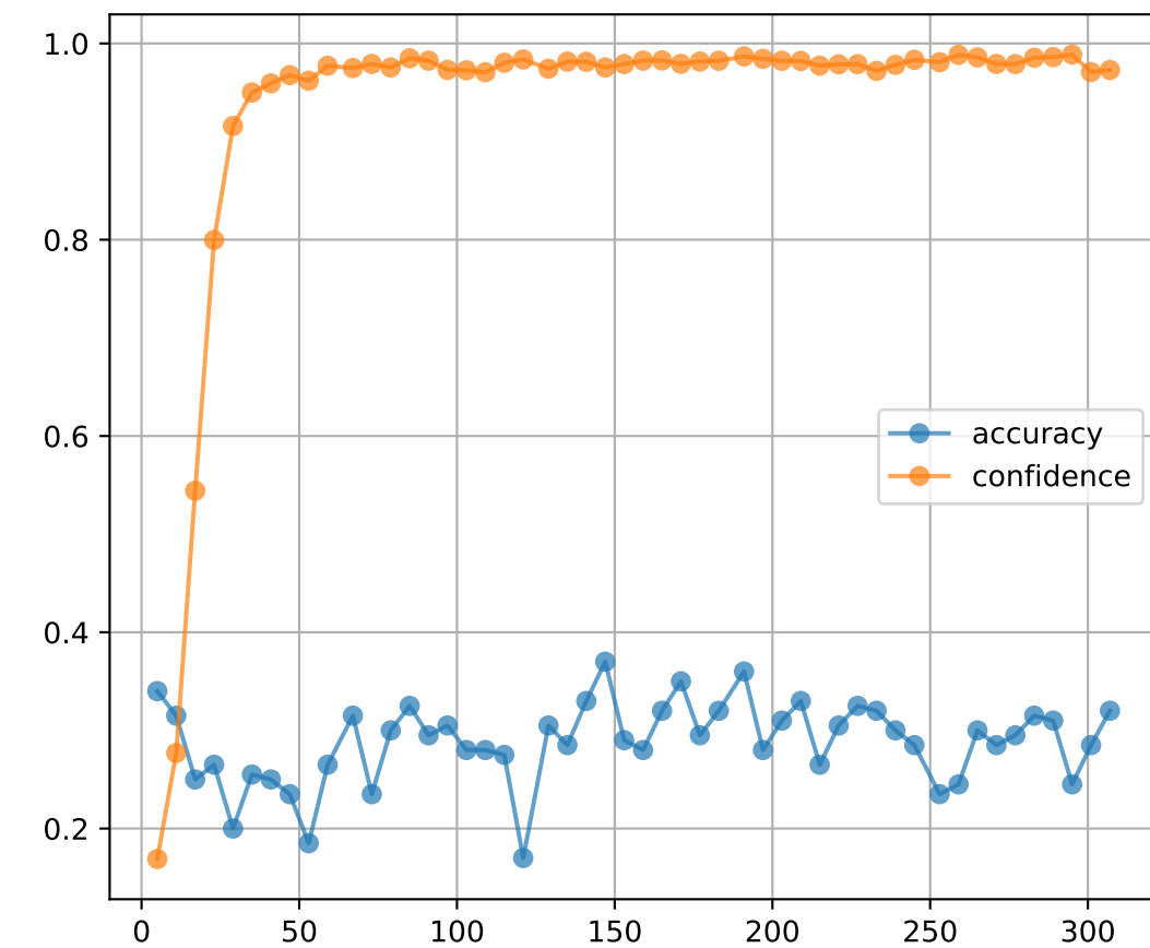
Evaluation Metrics
